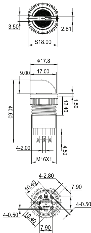
鍍金/銀引腳 Gold Plated Pins/Silver Contact
