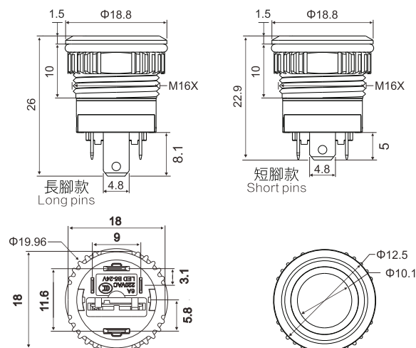
鍍銀長插腳 Silver Long Plated Pins
