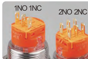
鍍金插腳，銀觸點 Gold Plated Pins/Silver Contact
