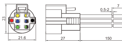
M5.1 / M5.2 / 5.4專用接插件 Connector
