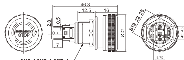
16/19/22M4急停 16/19/22M4 Stop Button
