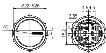
帶燈，大旋柄 LED,Big Handle
