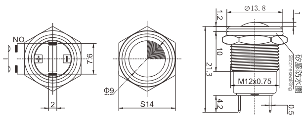
PBM12B外型尺寸 Outline Dimension
